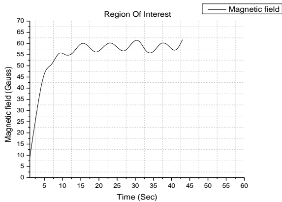
Fig.6. ROI magnetic sensor data graph
